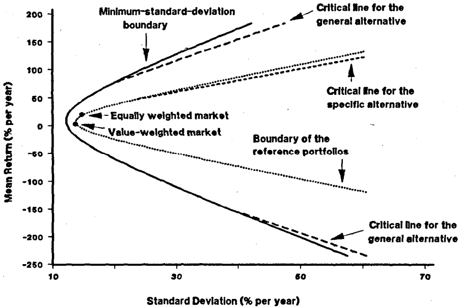
Figure 4 Likelihood-ratio tests of a single-beta pricing model against general and specific alternate hypotheses in the presence of a riskless asset
