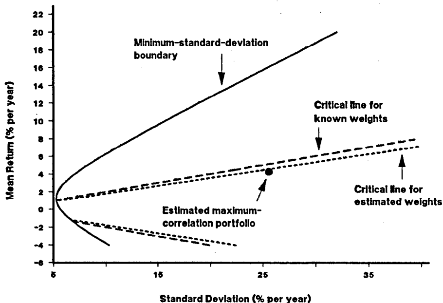
Figure 6 Likelihood-ratio tests of the consumption-beta model The tests are based on quarterly returns, in excess of a Treasury bill rate, and an Index of quarterly consumption growth. The sample minimum-standard-deviation boundary is constructed using 12 assets: 10 size-based portfolios plus a portfolio of long-term U.S. government bonds and a portfolio of bonds rated below Baa by Moody's. The critical lines reflect a 5 percent significance level. The critical line labeled "known weights" would be appropriate for testing the model with known weights in the portfolio having maximal correlation with consumption. The critical line labeled "estimated weights" is appropriate when the weights in the maximum-correlation portfolio are estimated. The pricing model is not rejected if the reference portfolio lies horizontally to the left of a critical line and to the right of the minimum-standard-deviation boundary.
